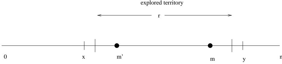
Figure 1: An exploration of two new edges in a phase needs at least r + 2 time units
