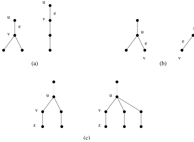
Figure 3: In (a) e is a red edge. In (b) e is a green edge. In (c) all solid edges are blue.
